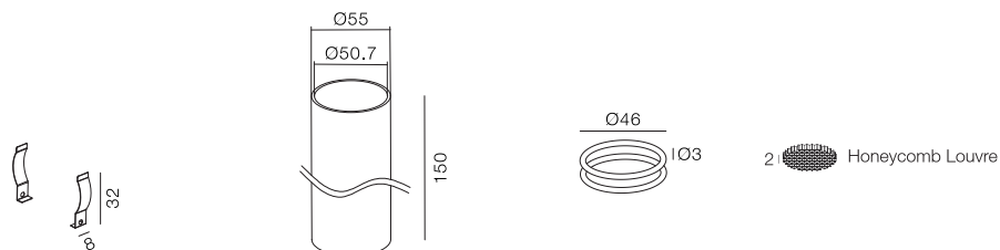
Optional spring mounting
